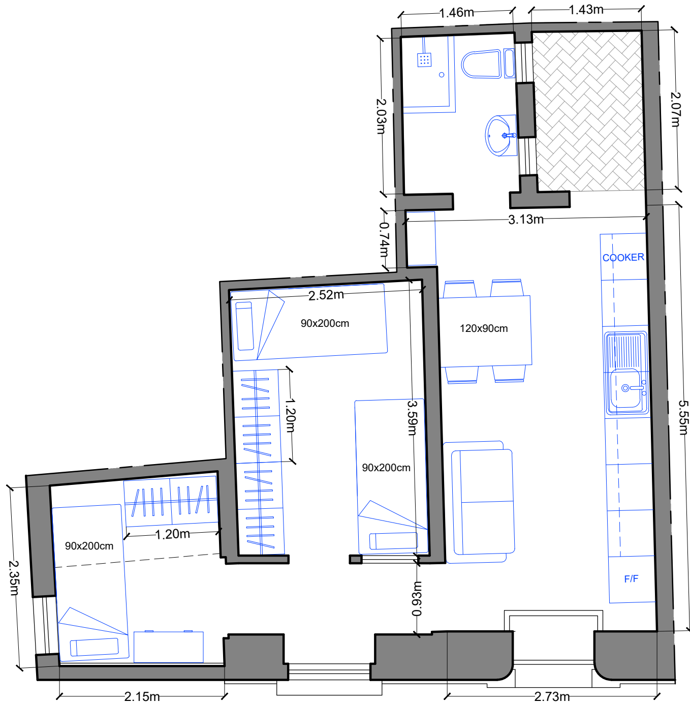
Proposed Ground Floor Level Scale 1:50
